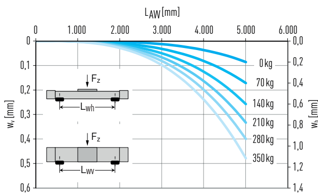
Fig. 11.2 Deflection w over unsupported axle length L_{\text{AW}} under payload F_z
