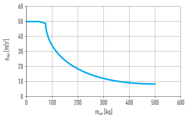
Fig. 11.1 Max. Acceleration a_{\text{max}} as a function of the external payload m_{\text{ext}}
