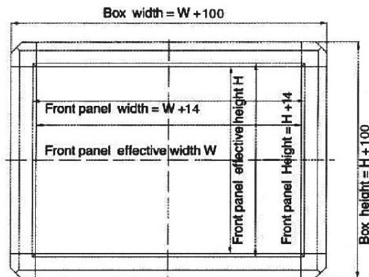
box dimensions (without a handle)
