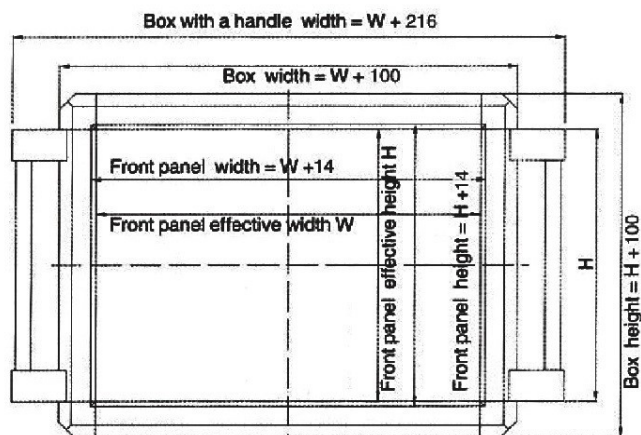
Box dimensions (with handles on both sides)
